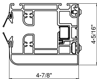
TRACK DETAIL
