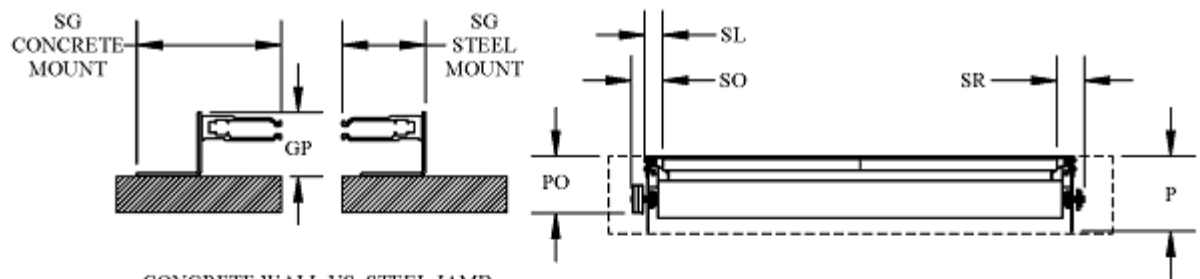
CONCRETE WALL VS. STEEL JAMB MOUNTING
